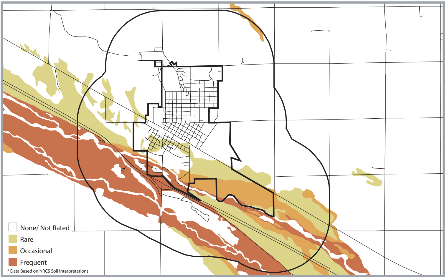
Map 3.2 Flood Frequency
