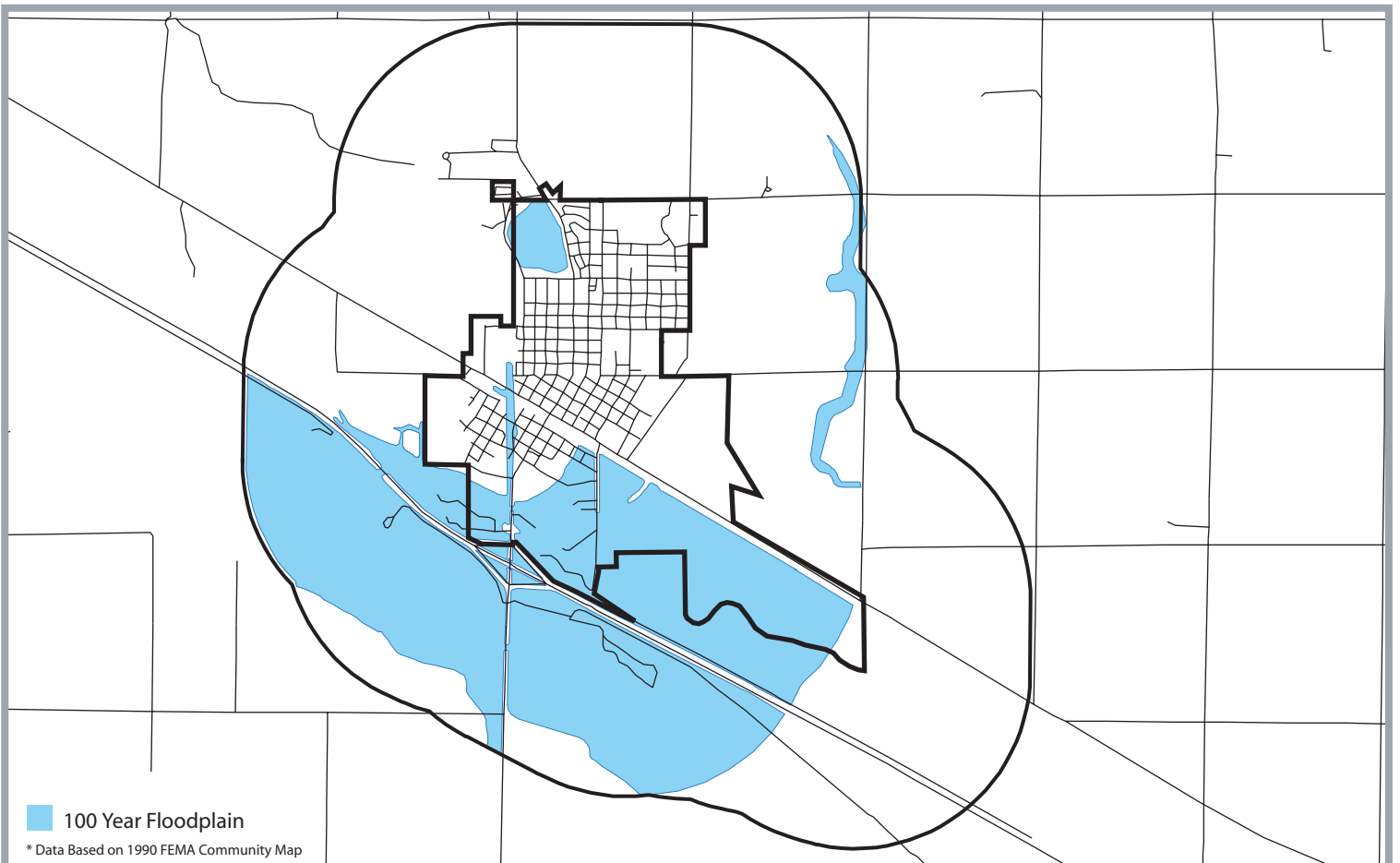
Map 3.3 FEMA Floodplain
